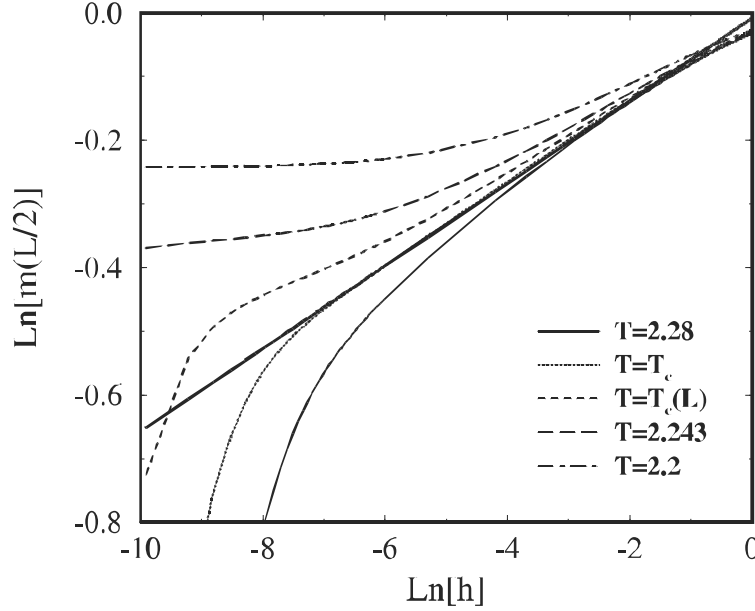
Fig. 3. Field dependence of the magnetization in the center of the strip of width L = 200 at several temperatures around the infinite system critical temperature T_c .
