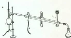
Destillations-Apparate
