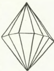
Dihexagonale Pyramide
