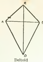
Deltoid
