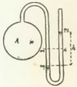
Heber-Manometer
