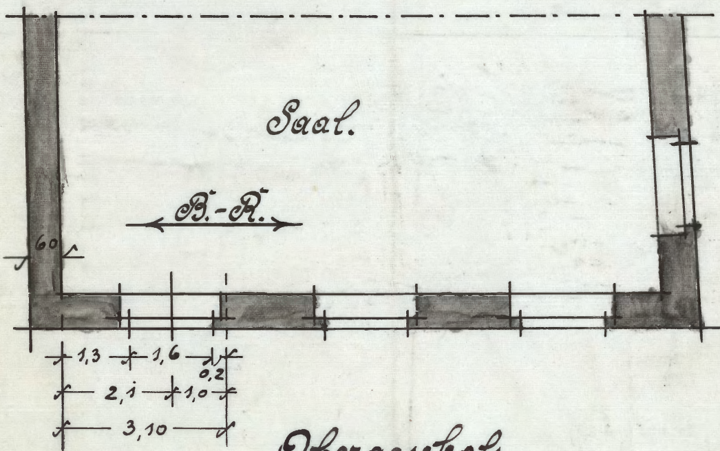
Erdgeschoss.
