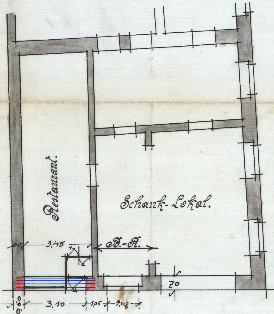
Erdgeschoss.
