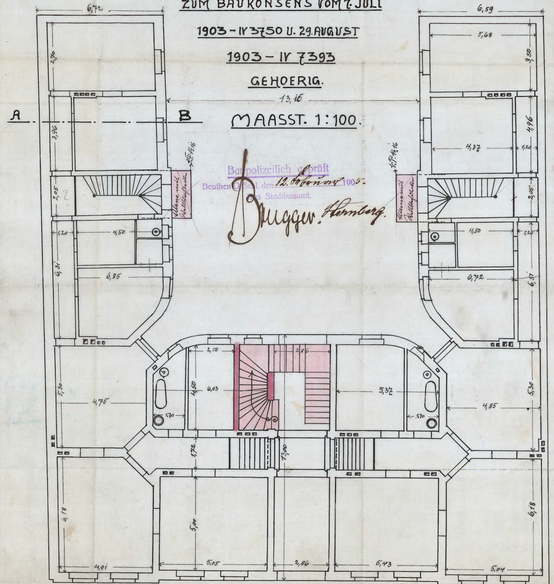
ERDGESCHOSS.
