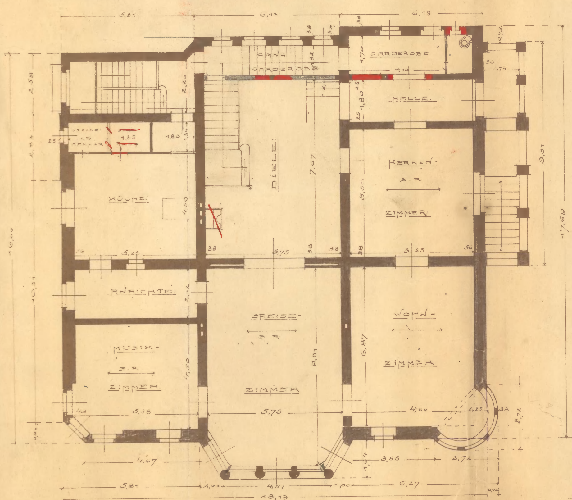
ERDGESCHOSS.
