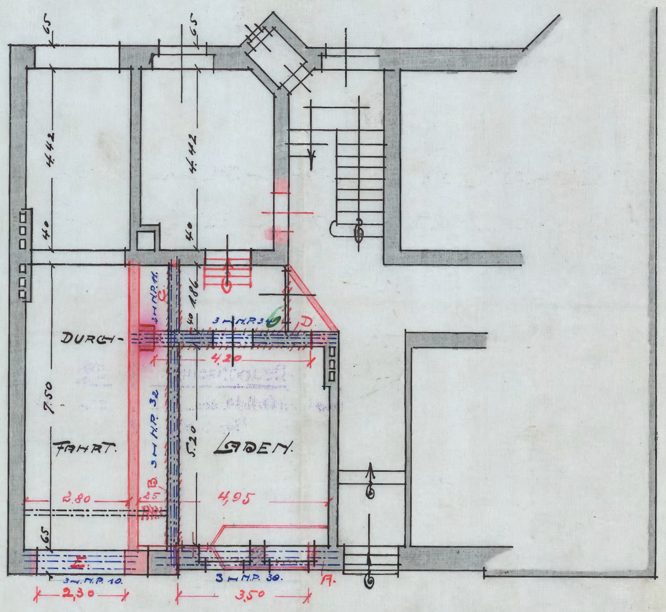
ERDGESCHOSS.
